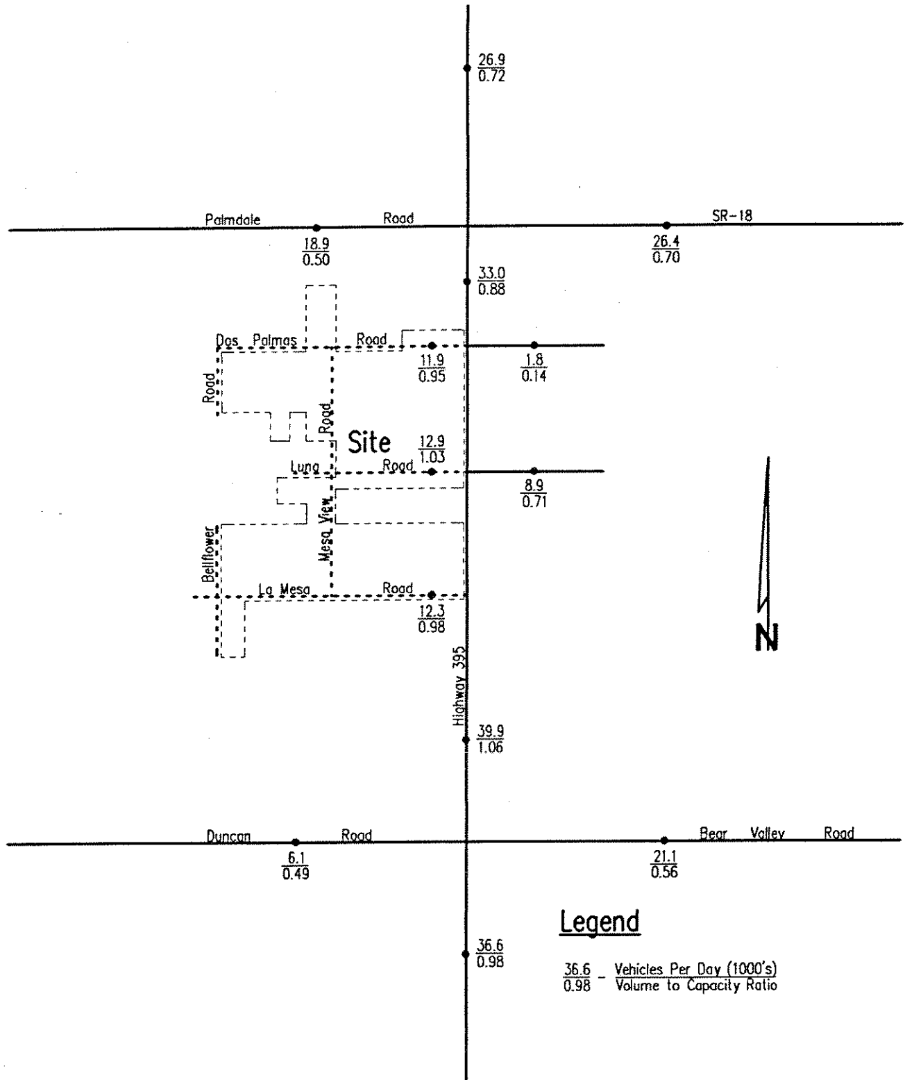
Figure 9 1999 Cumulative Daily Volumes and Volume to Capacity Ratios
