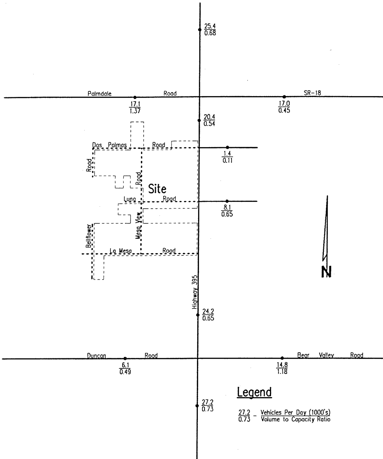
Figure 8 1999 Background Plus Other Development Daily Volumes and Volume to Capacity Ratios
