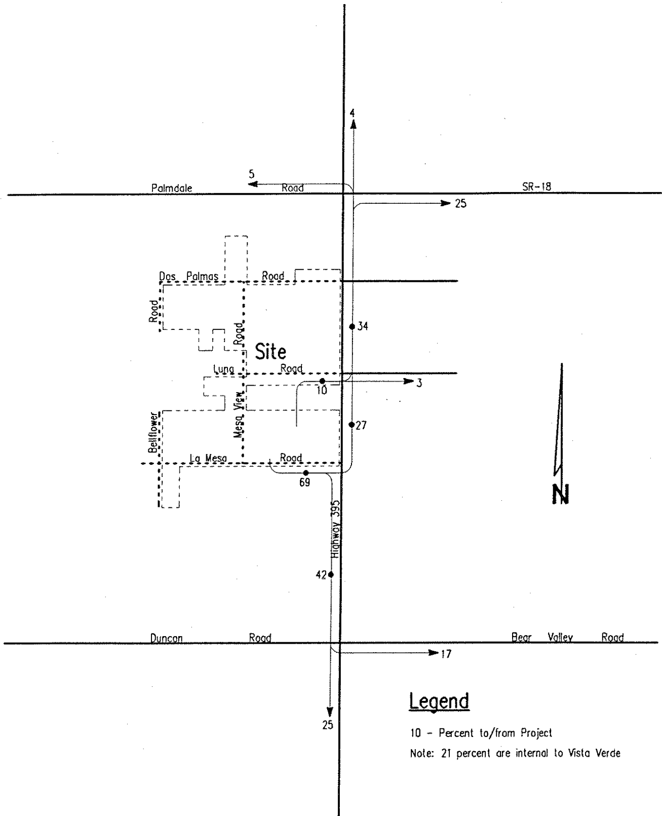
Figure 5g Zone 7 Traffic Distribution
