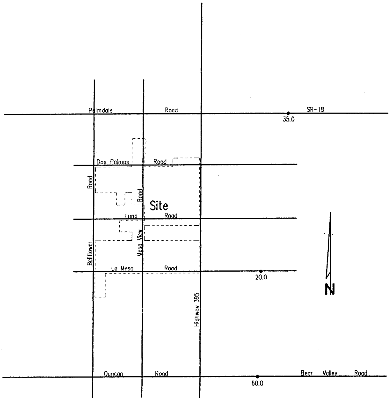
Figure 10 Future Daily Traffic Volumes
