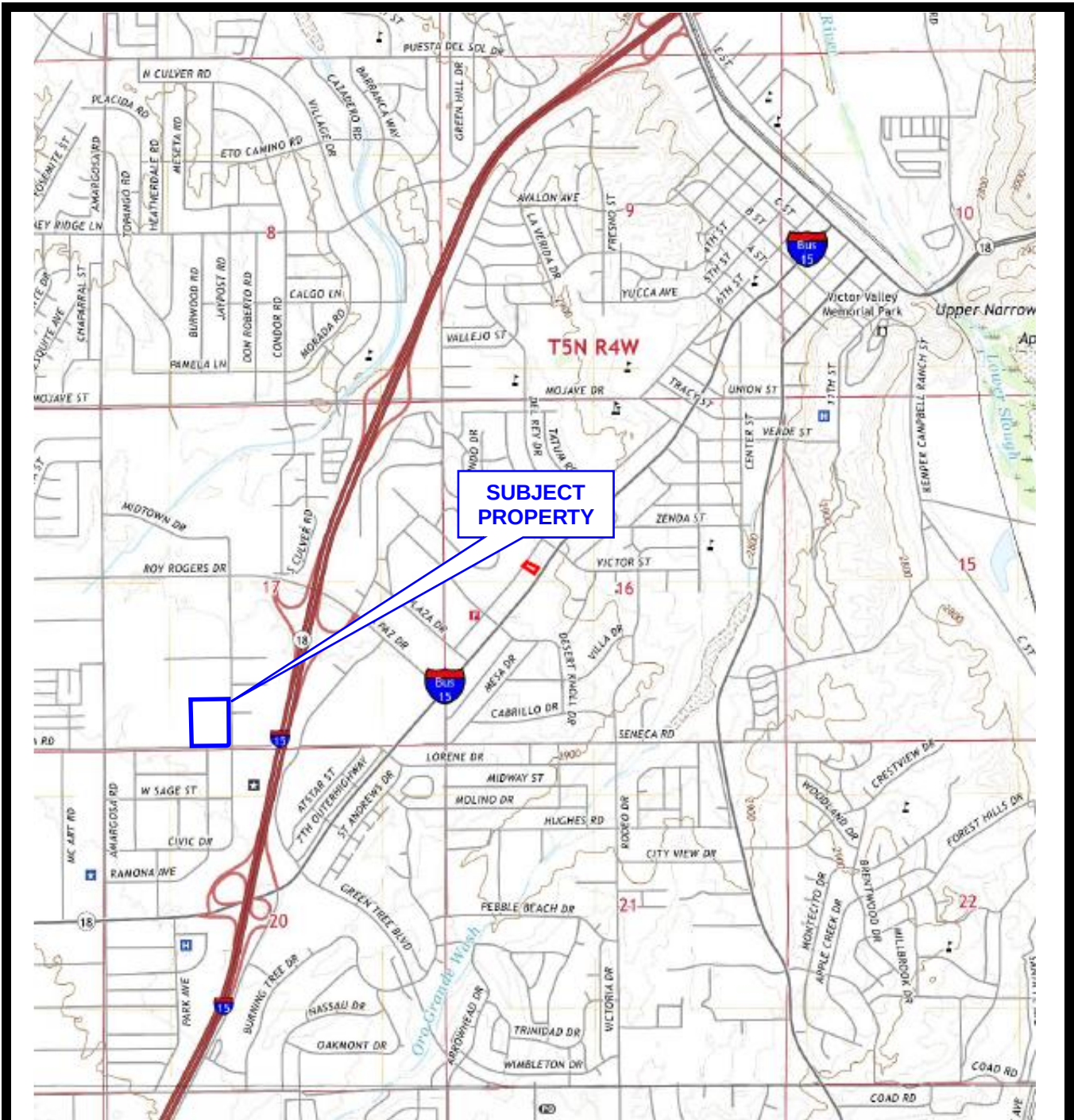
Figure 1: Victorville Topographic Map
